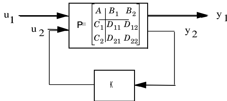
Figure 10-8: \mathbf{H}_\infty control system CL = \text{lft}(P, K) = T_{y_1 u_1} .
